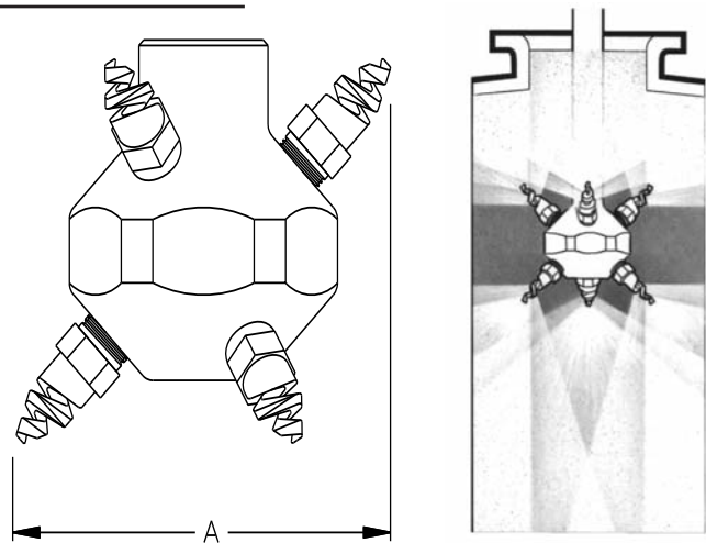
Typical LEM installation
